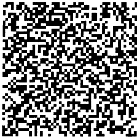
Fig. 3. A hypothetical 200 pixels×200 pixels landscape map for which lacunarity=1.2334 at the 2 pixels×2 pixels level (Table 1).
